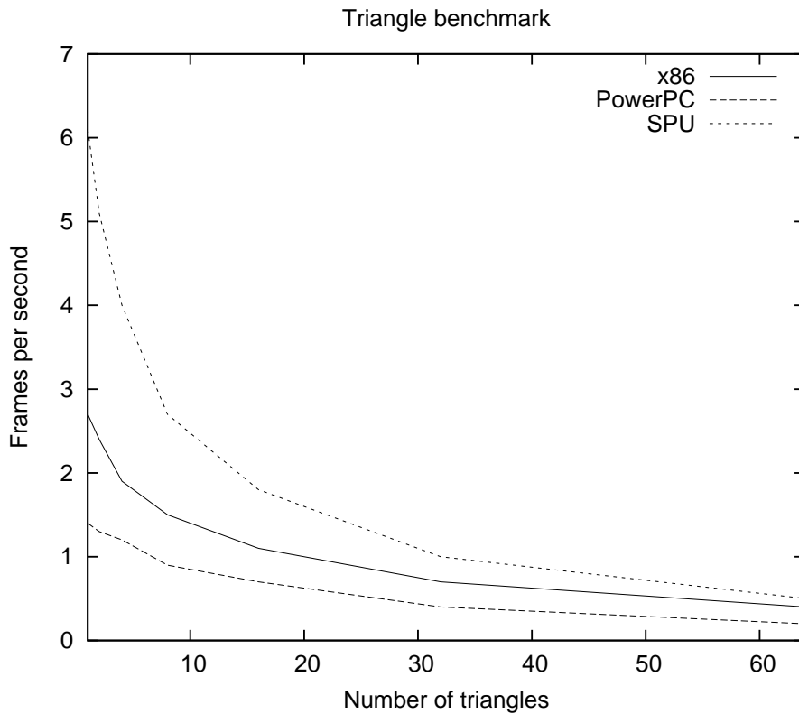
Figure 2: Triangle Benchmark Triangle
