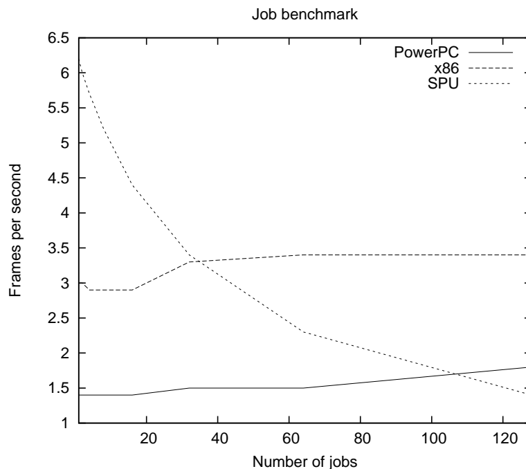
Figure 1: Job Benchmark
